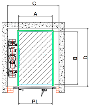
Entrada Unilateral
