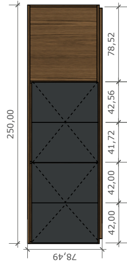
13 VISTA FRONTAL - BALCÃO COFFEE BREAK 1:2,25
