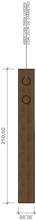
12 VISTA SUPERIOR - BALCÃO COFFEE BREAK 1:1,25
